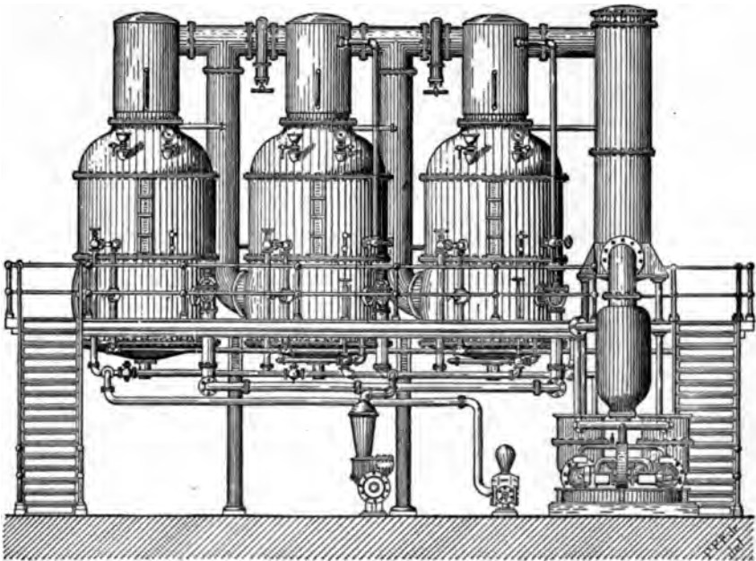
FIG. 73.—MULTIPLE-EFFECT EVAPORATING APPARATUS.—( Farmers' Bulletin 52. )
